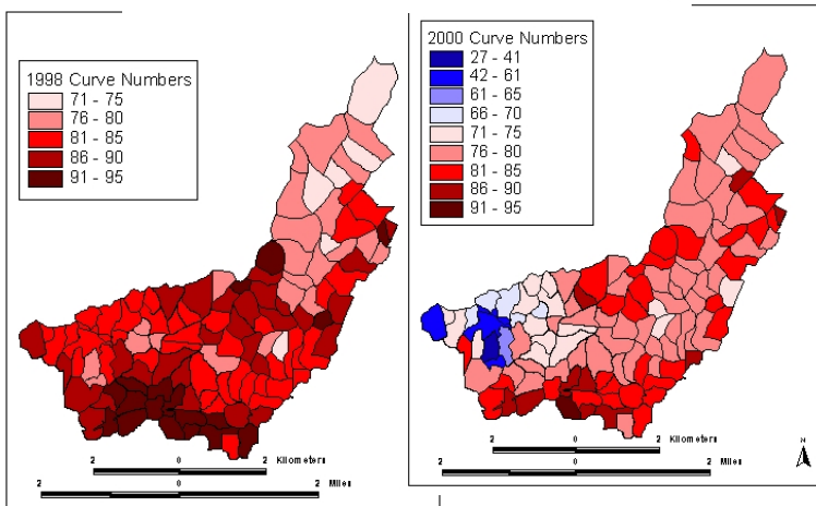
Curve Numbers per Subbasin for Years 1998 (from consultant; based on land use) and 2000 (from Remote Sensing imagery; based on land cover)
